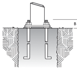
BASE MOUNT OPTION
